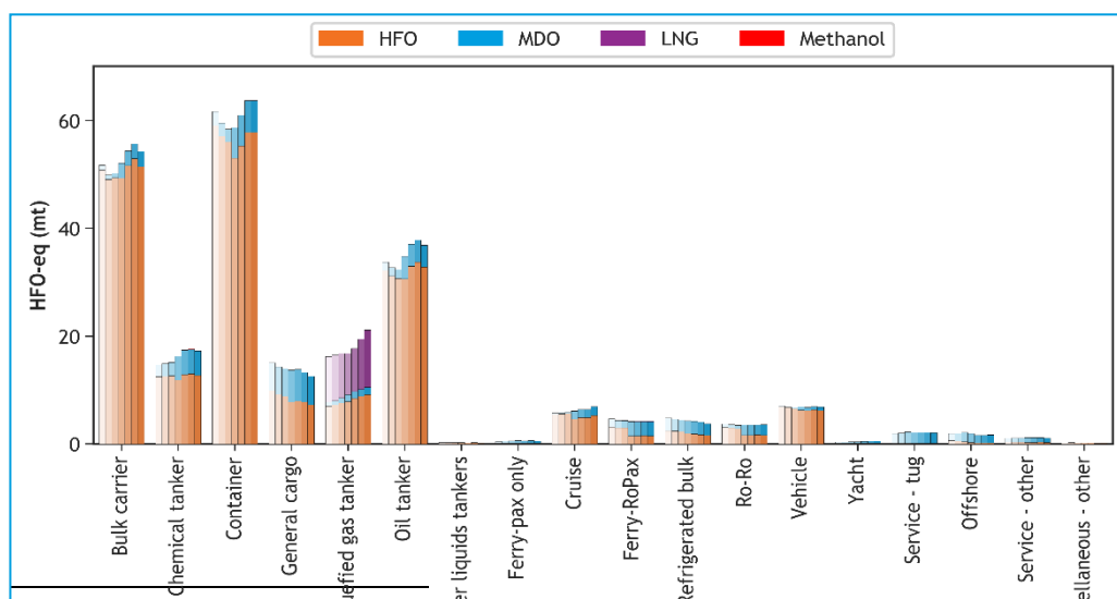
Figure 4 – International HFO-equivalent fuel consumption per ship type, according to the voyage-based allocation of international emissions
